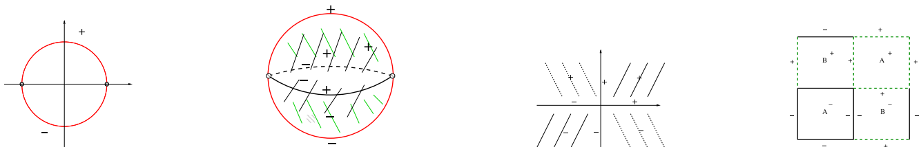
FIG. 3. The \mathbb{Z}_2 -CW decompositions of (a) \mathbb{S}^{1,1} , (b) \mathbb{S}^{1,2} , with 2 0-cells, 4 1-cells and 4 2-cells, corresponding to the one-point compactification of \mathbb{R}^{0,2} decomposed into quadrants and half lines depicted in (c), and (d) the decomposition of \mathbb{T}^2 .
