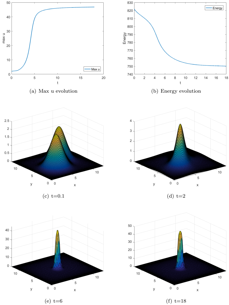
FIGURE 8. Example 6. Simulation of Keller-Segel equations with initial condition (5.10)
