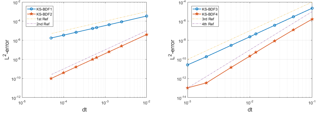
(a) BDF1 and BDF2 for Keller-Segel with known exact solution (b) BDF3 and BDF4 for Keller-Segel with known exact solution
