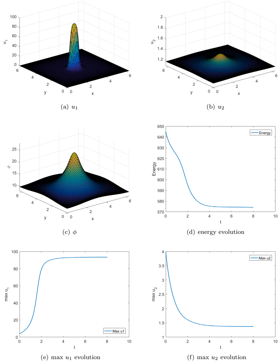
FIGURE 10. Example 7. Simulation with \chi_2 = 0.01
