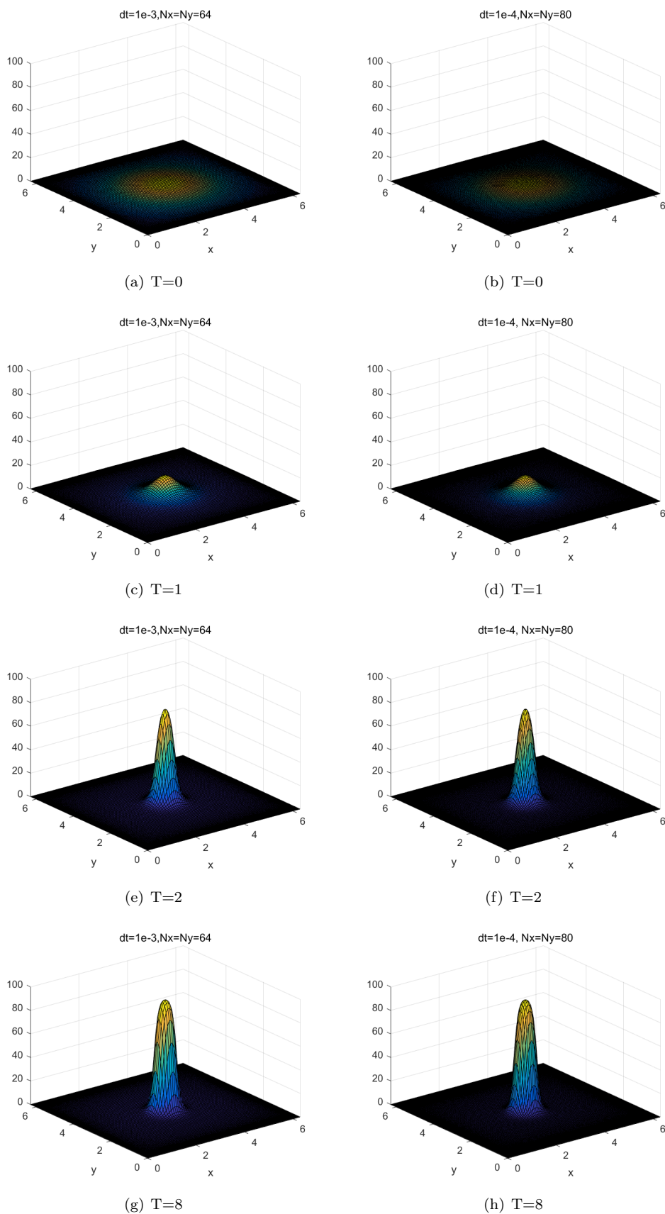
FIGURE 6. Example 5. Simulation of Keller-Segel equations with chemotaxis.
