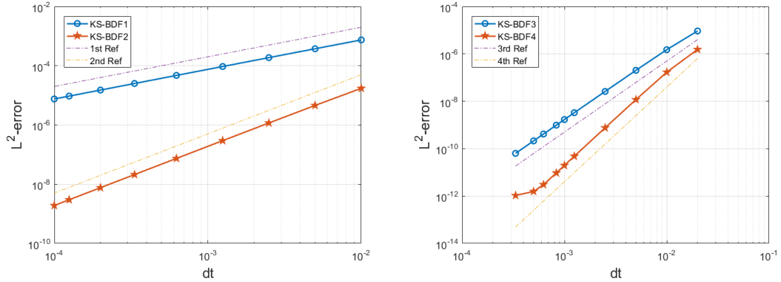
(c) BDF1 and BDF2 for Keller-Segel with unknown exact solution (d) BDF3 and BDF4 for Keller-Segel with unknown exact solution
