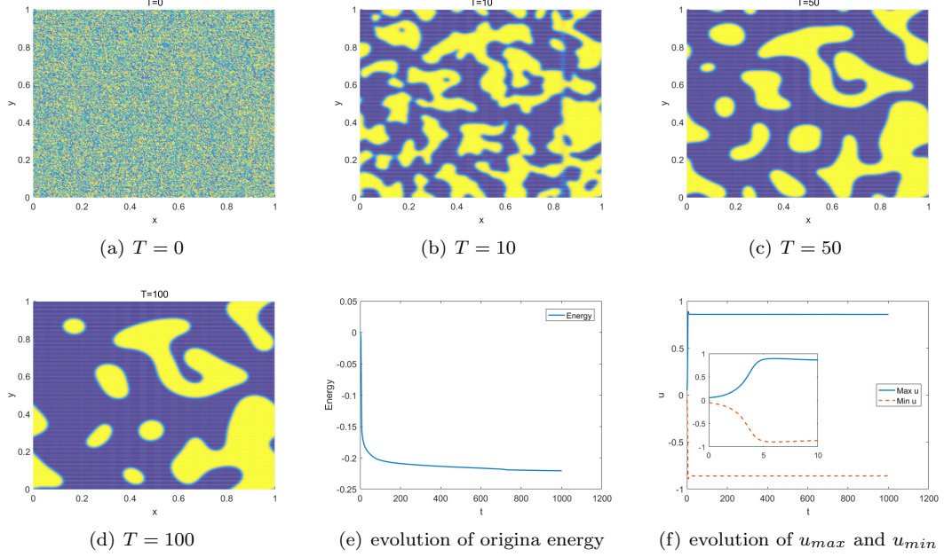
FIGURE 2. Example 1. Spinodal decomposition by the Allen-Cahn equation. The simulation is obtained with \delta t = 0.001 using the scheme (2.6)-(2.10).
