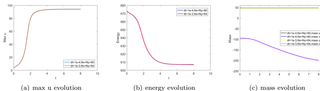
FIGURE 7. Example 5. Simulation of Keller-Segel equations with chemotaxis.
