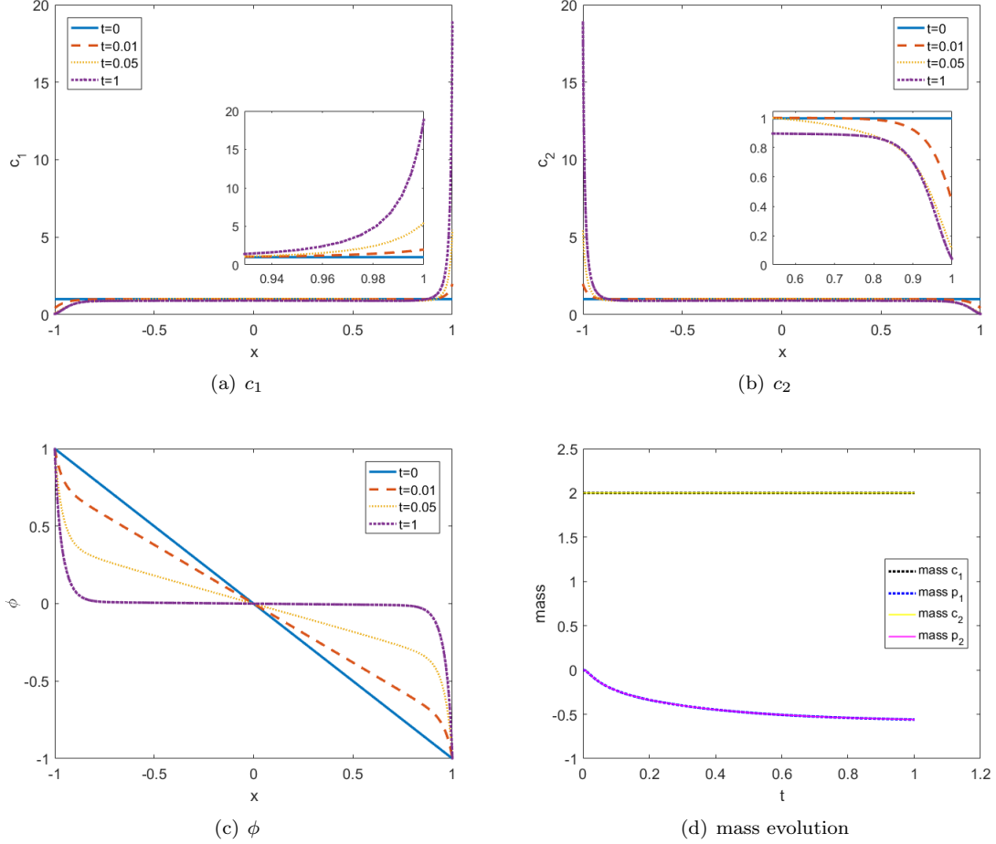
FIGURE 4. Example 3. Gouy-Chapman model: Profiles of c_1, c_2 and \phi
