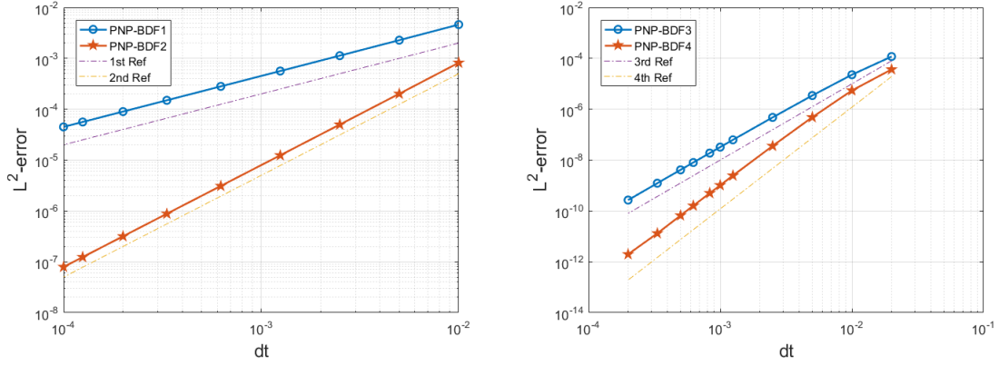
(c) BDF1 and BDF2 for PNP with unknown exact solution (d) BDF3 and BDF4 for PNP with unknown exact solution
