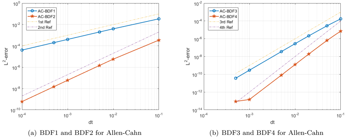
FIGURE 1. ( Example 1. ) Accuracy test for the Allen-Cahn equation using the new SAV/BDF k schemes ( k = 1, 2, 3, 4 ).
