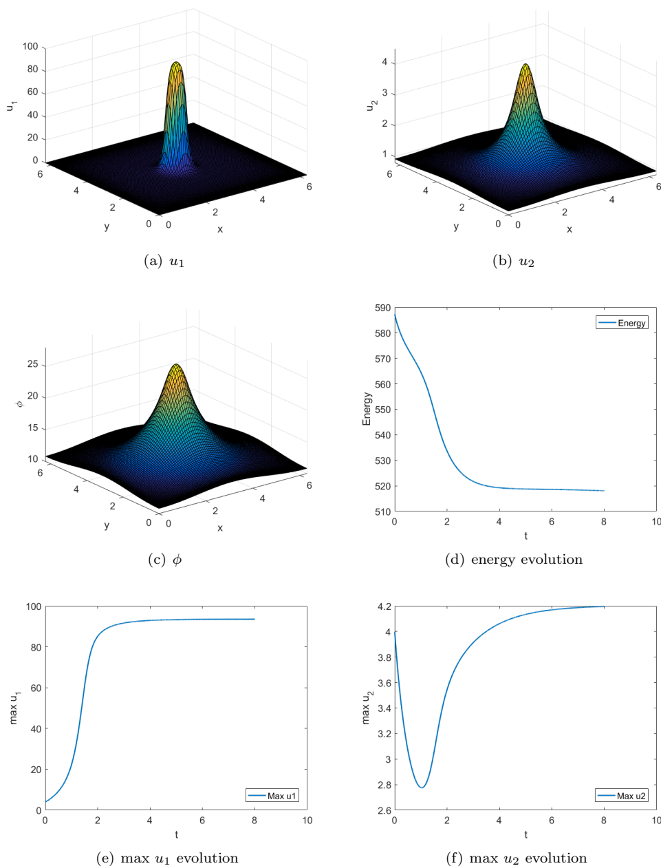
FIGURE 9. Example 7. Simulation with \chi_2 = 0.1
