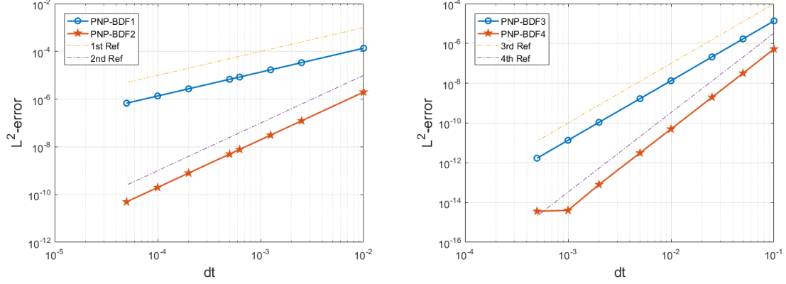
(a) BDF1 and BDF2 for PNP with known exact solution (b) BDF3 and BDF4 for PNP with known exact solution
