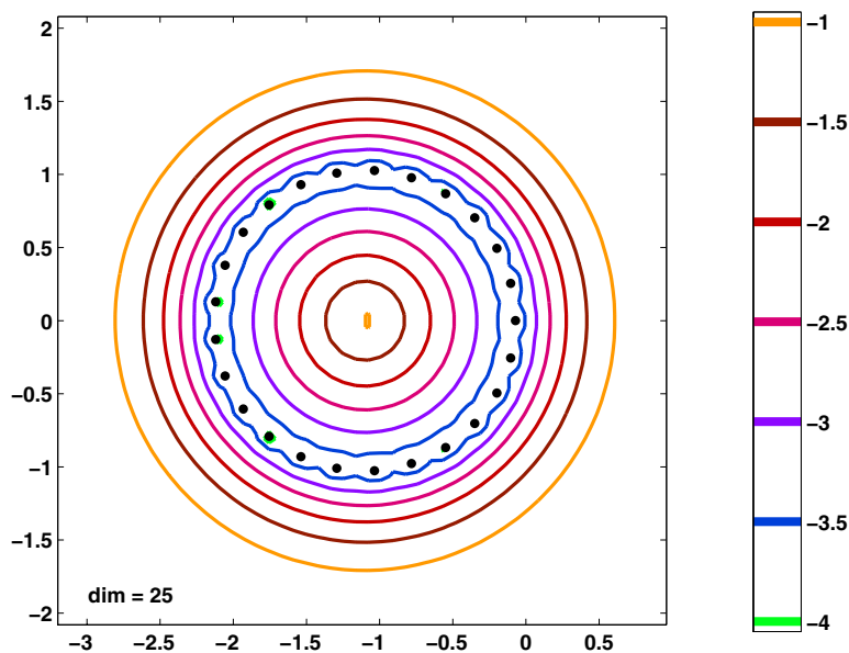
Fig. 4 \epsilon -pseudospectra for the transient example.
